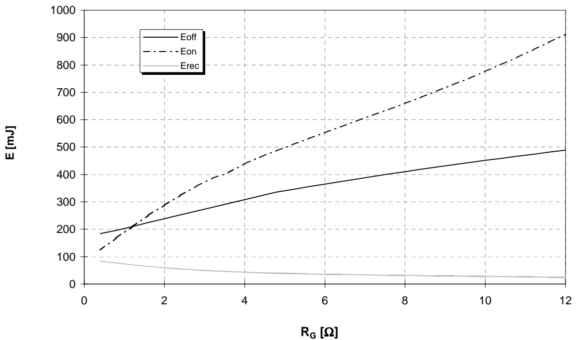
Schaltverluste (typisch) E_{on} = f(R_G), E_{off} = f(R_G), E_{rec} = f(R_G) Switching losses (typical) I_C = 1200A, V_{CE} = 600V, T_j = 125^\circ C
