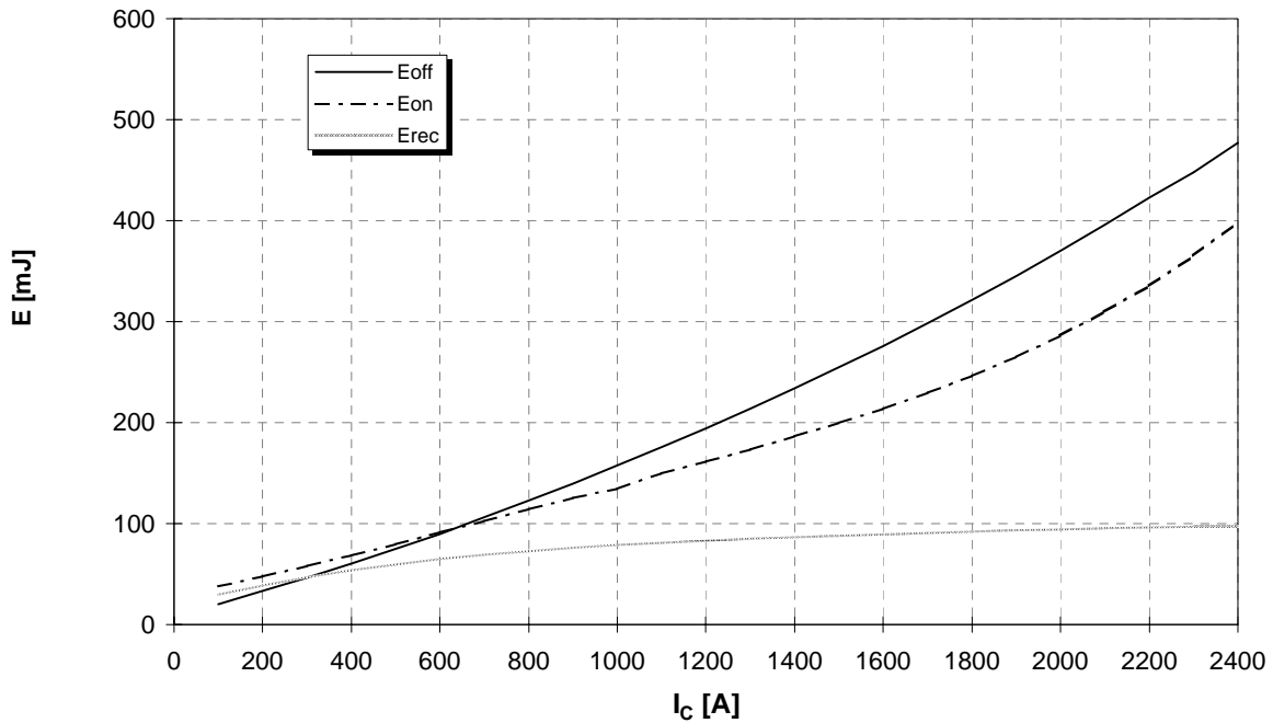
Schaltverluste (typisch) E_{on} = f(I_C), E_{off} = f(I_C), E_{rec} = f(I_C) Switching losses (typical) R_{gon} = R_{goff} = 0,82 \Omega, V_{CE} = 600V, T_j = 125^\circ C
