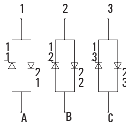
Three phase AC switches half controlled
