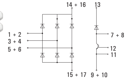
Three phase diodes bridges with integrated brake chopper
