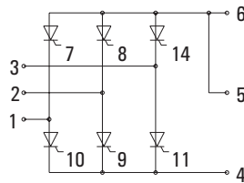
Three phase bridges fully controlled
