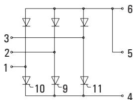
Three phase bridges half controlled
