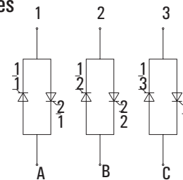
Three phase AC switches half controlled
