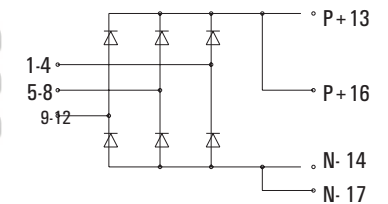
Three phase diodes bridges with integrated brake chopper
